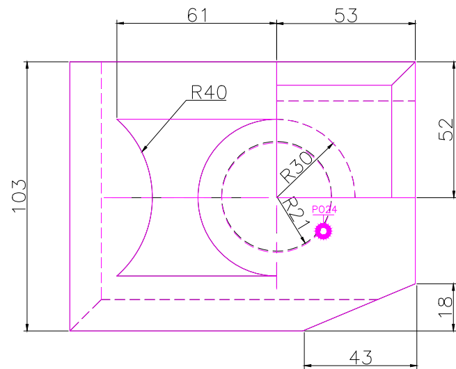
TOP SCALE 1/2
