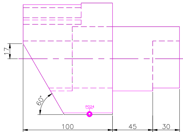
FRONT SCALE 1/2
