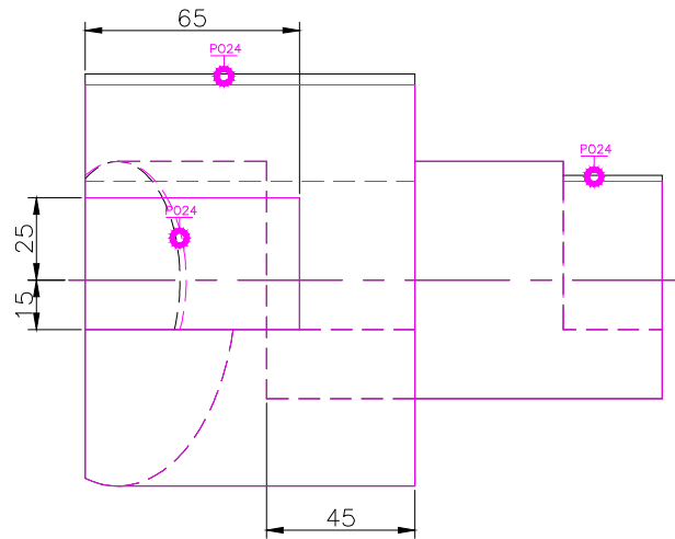
TOP SCALE 1/2
