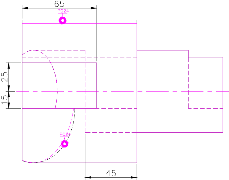
TOP SCALE 1/2
