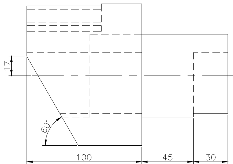
FRONT SCALE 1/2
