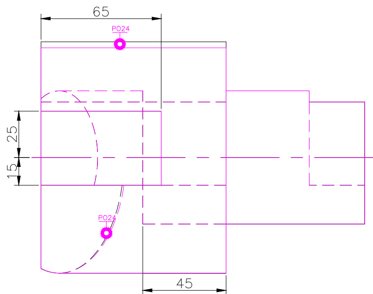
TOP SCALE 1/2
