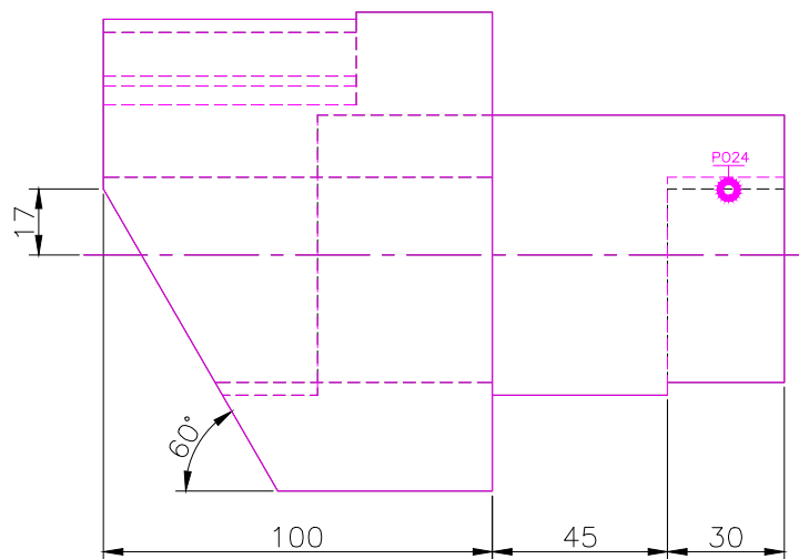
FRONT SCALE 1/2
