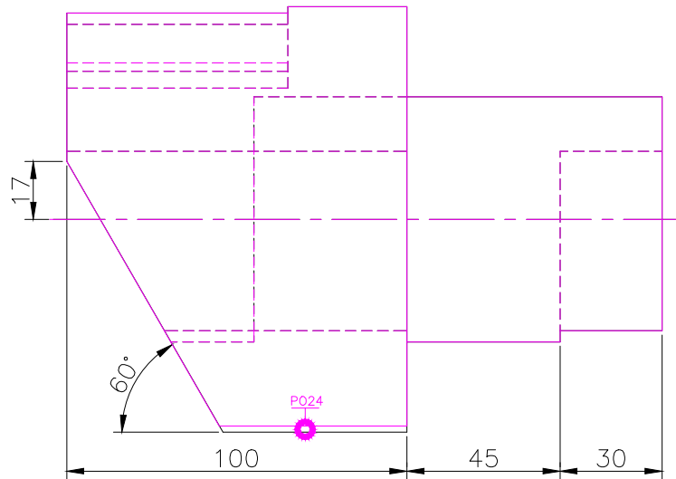
FRONT SCALE 1/2
