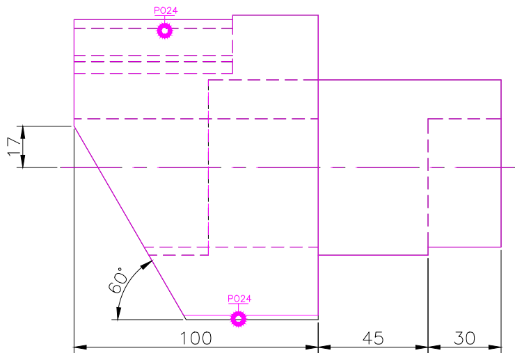
FRONT SCALE 1/2
