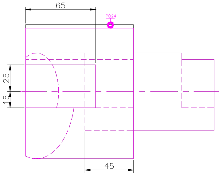
TOP SCALE 1/2
