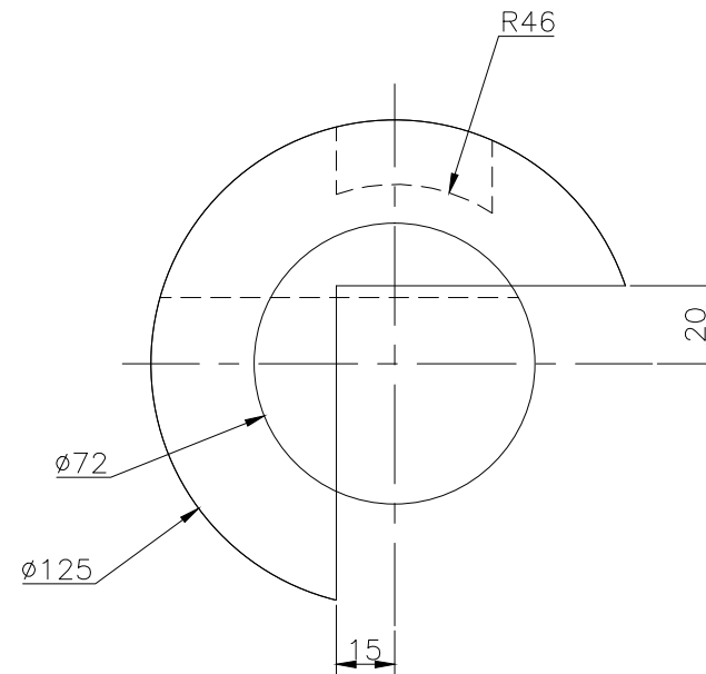
RIGHT SCALE 1/2
