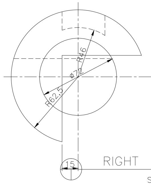
FRONT SCALE 1/2
