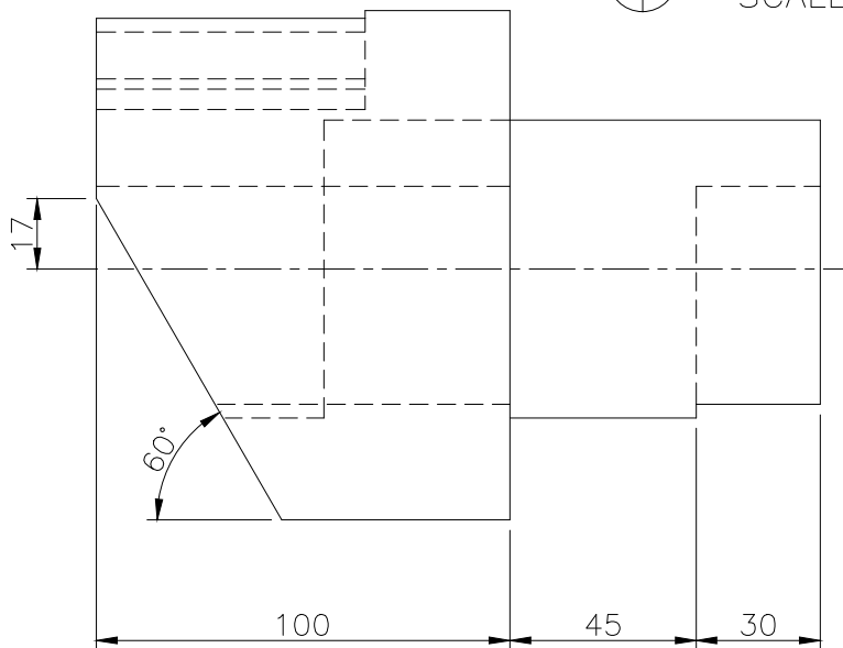
FRONT SCALE 1/2
