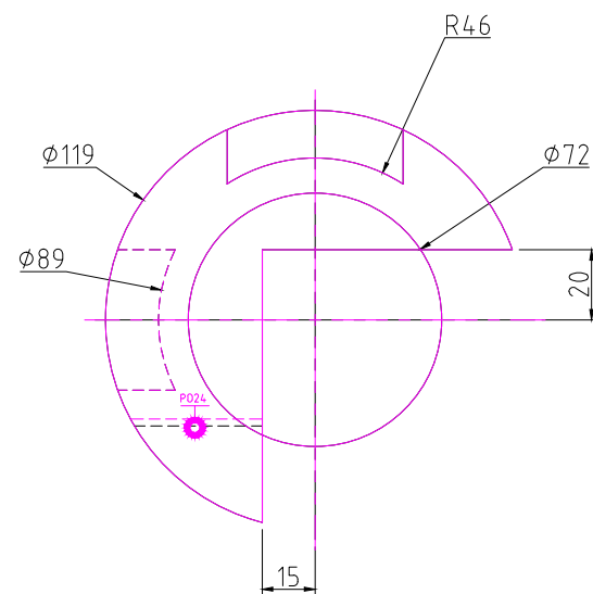
RIGHT SCALE 1/2
