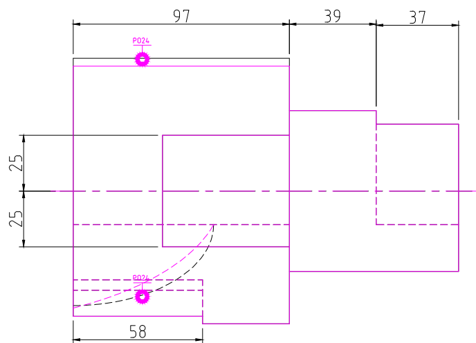
TOP SCALE 1/2
