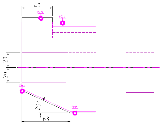
FRONT SCALE 1/2
