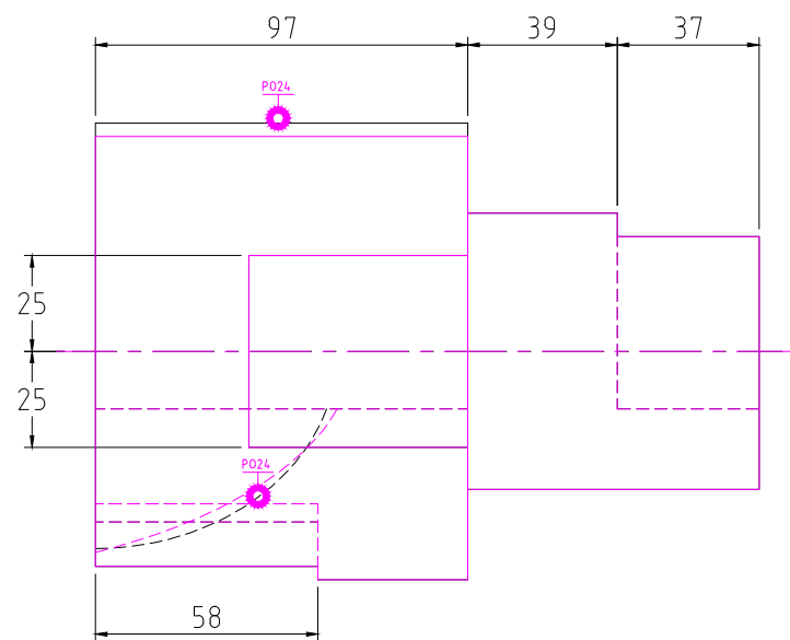
TOP SCALE 1/2
