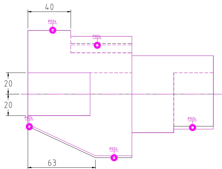
FRONT SCALE 1/2
