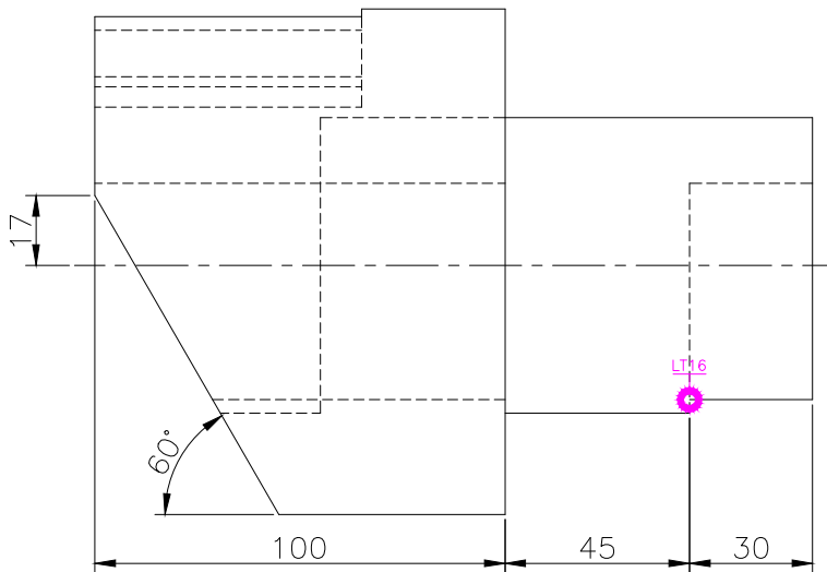
FRONT SCALE 1/2
