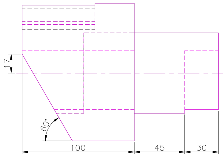
FRONT SCALE 1/2
