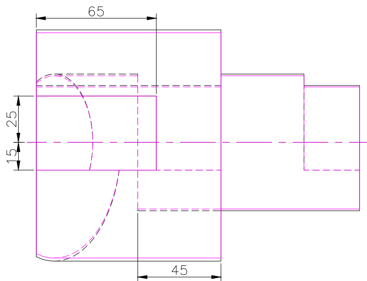
TOP SCALE 1/2
