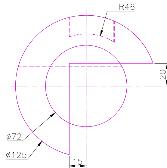
RIGHT SCALE 1/2
