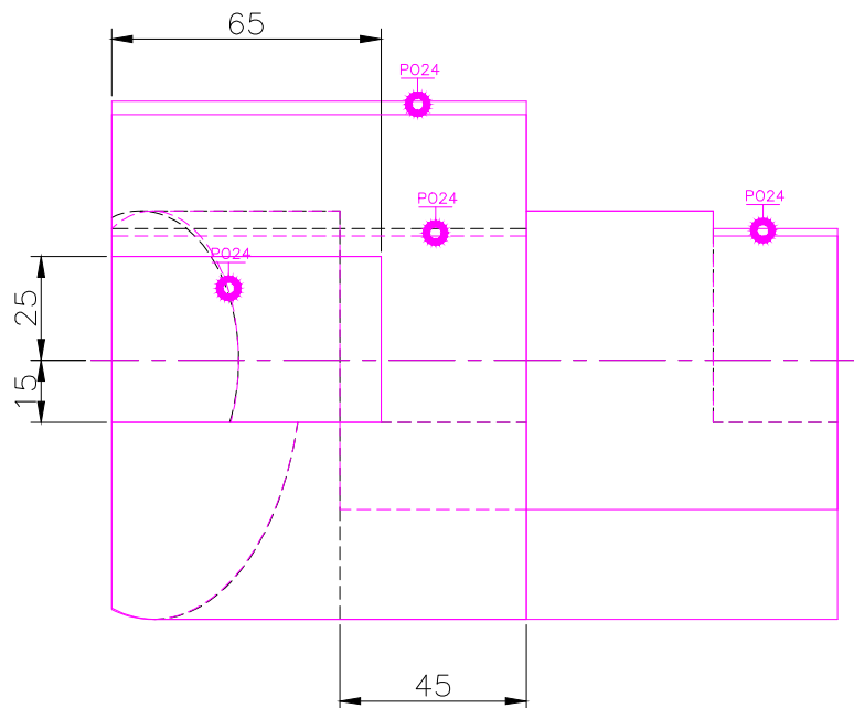
TOP SCALE 1/2
