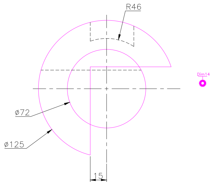
RIGHT SCALE 1/2
