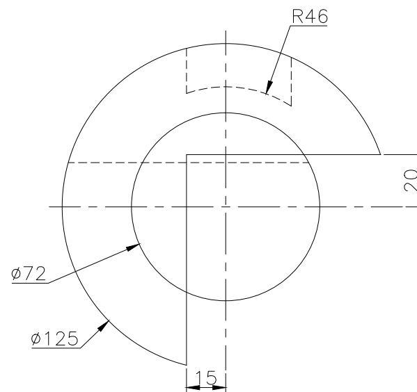
RIGHT SCALE 1/2
