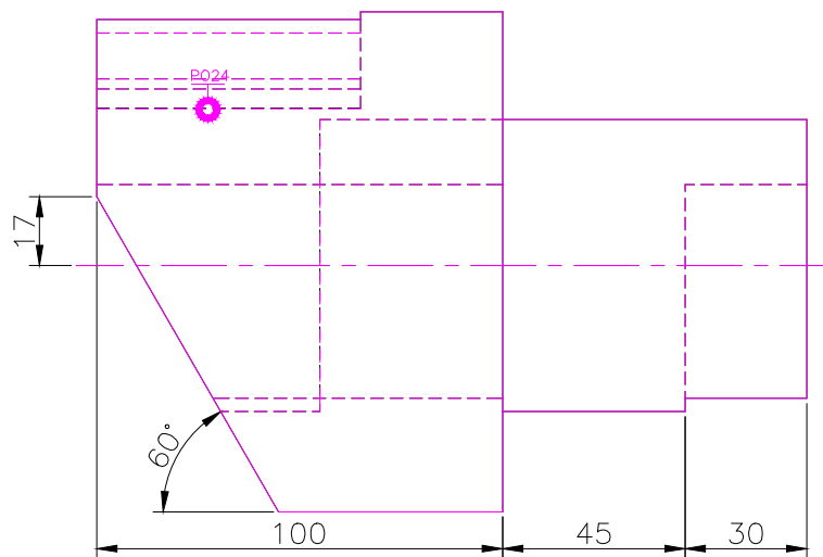
FRONT SCALE 1/2
