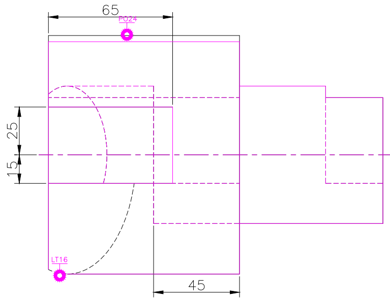
TOP SCALE 1/2
