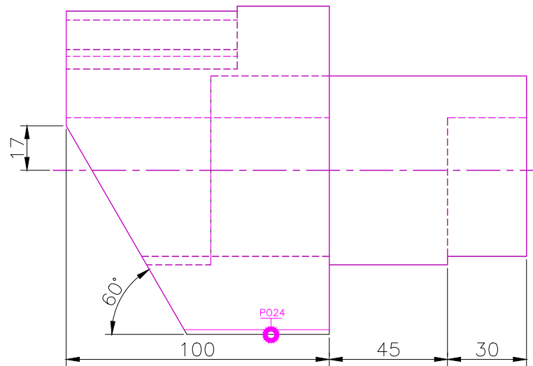
FRONT SCALE 1/2
