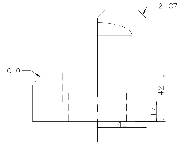
RIGHT SCALE 1/2
