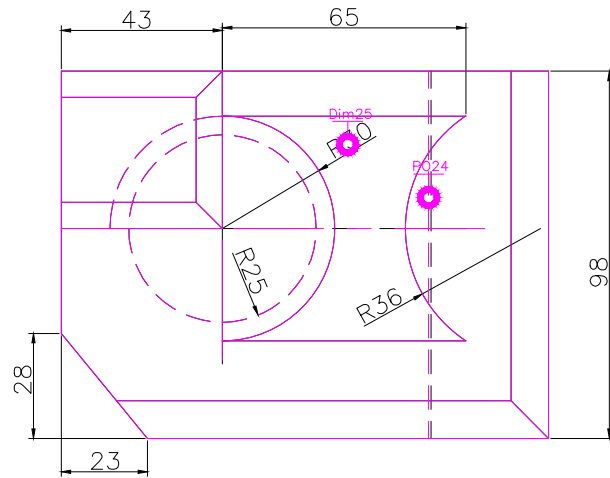
TOP SCALE 1/2
