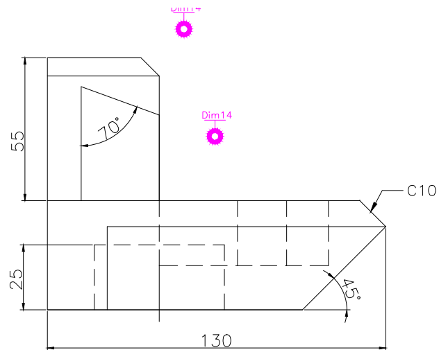
FRONT SCALE 1/2
