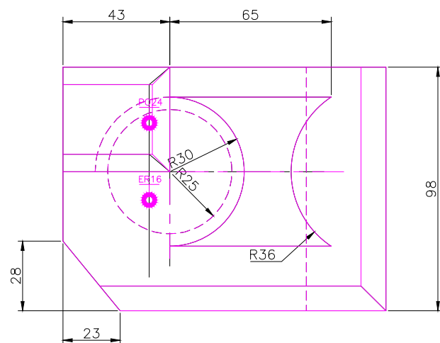
TOP SCALE 1/2
