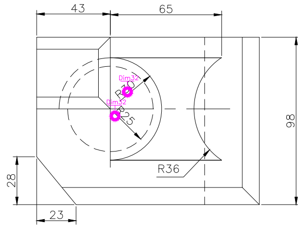
TOP SCALE 1/2
