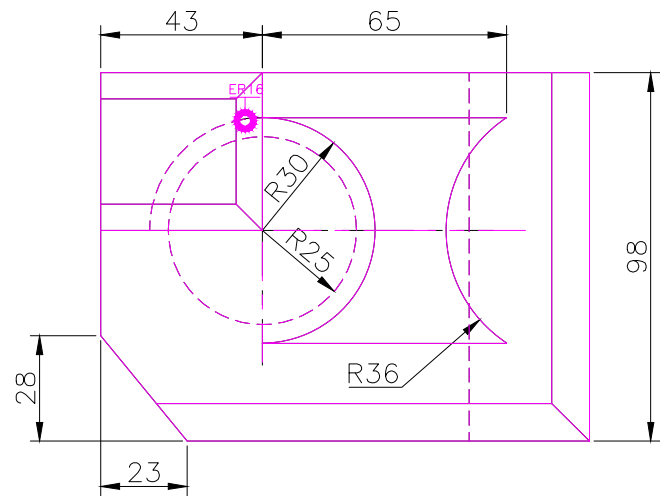
TOP SCALE 1/2
