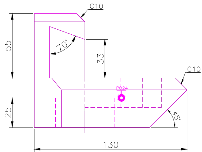
FRONT SCALE 1/2
