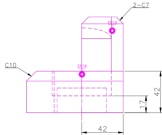
RIGHT SCALE 1/2
