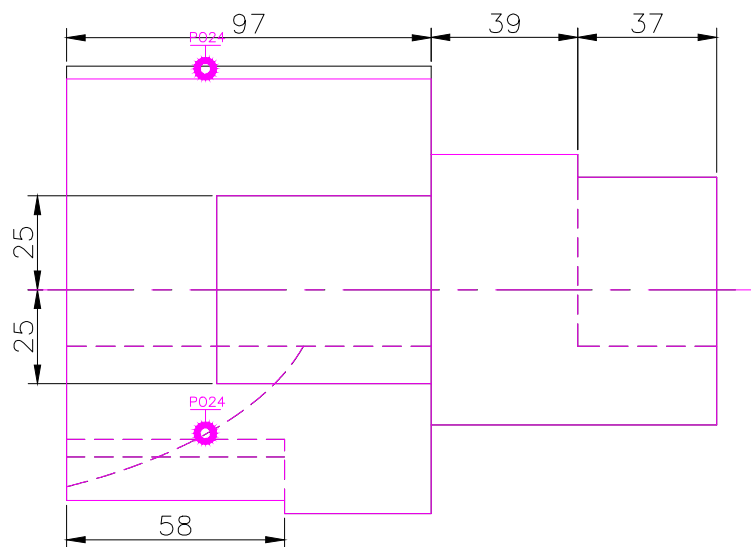
TOP SCALE 1/2
