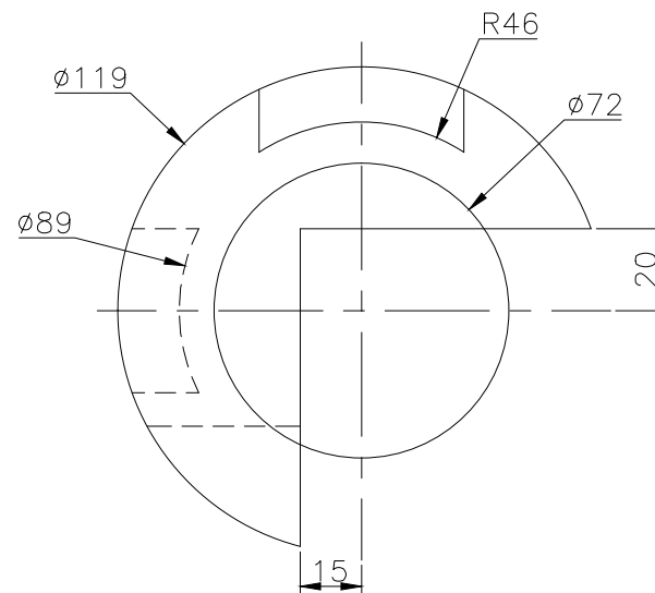
RIGHT SCALE 1/2
