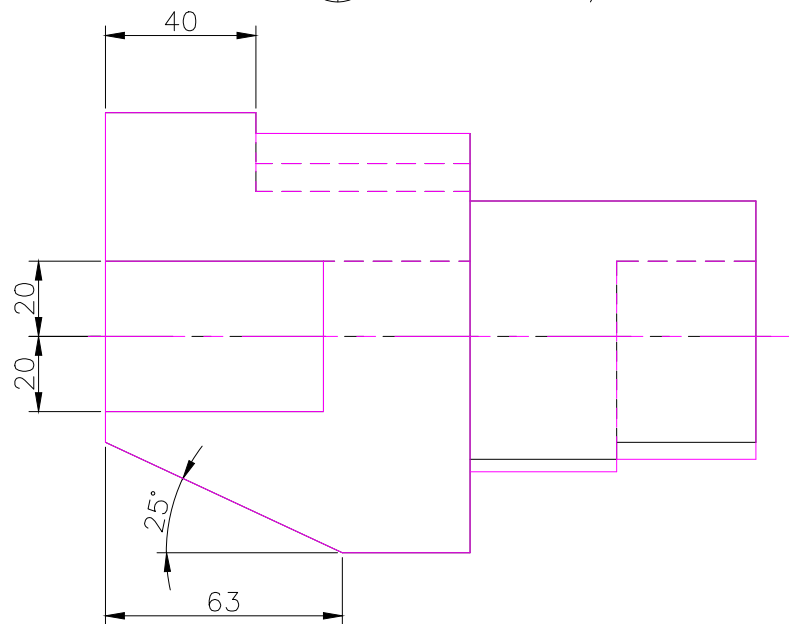
FRONT SCALE 1/2
