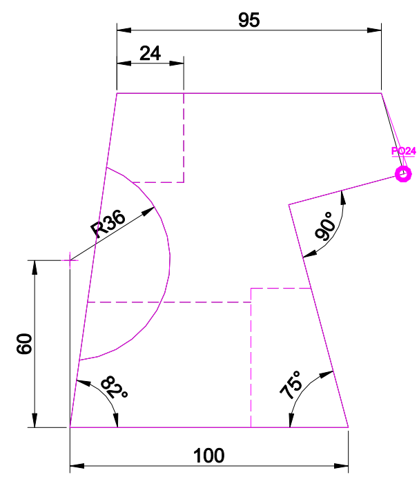
RIGHT SCALE 1/2
