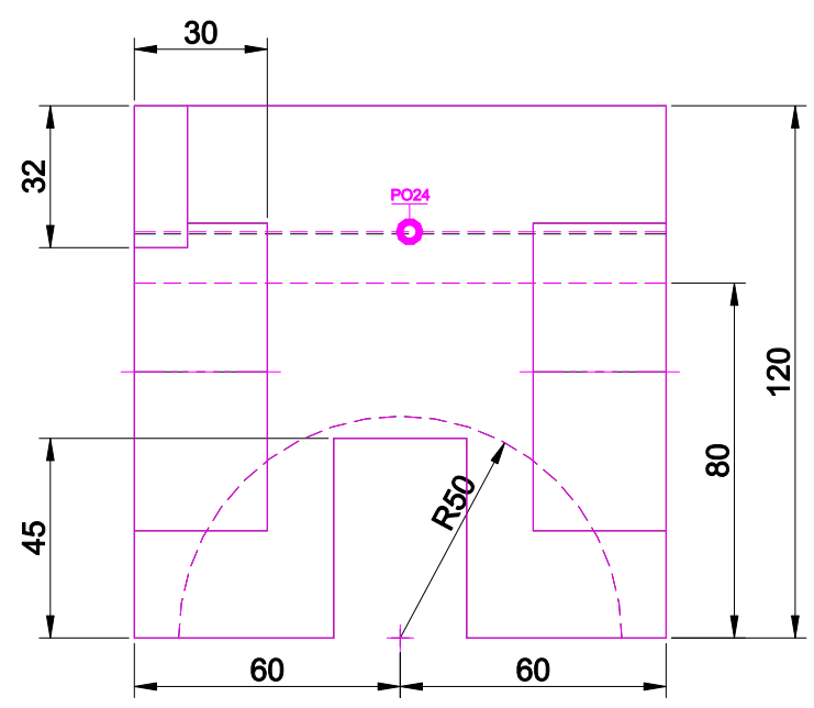
FRONT SCALE 1/2
