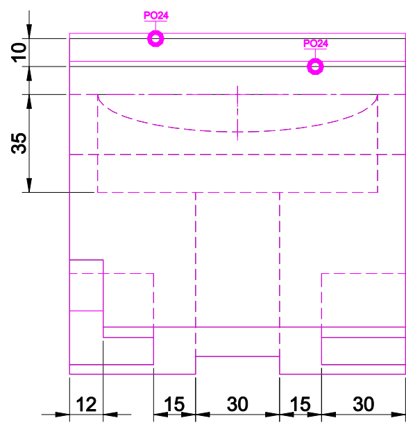
TOP SCALE 1/2
