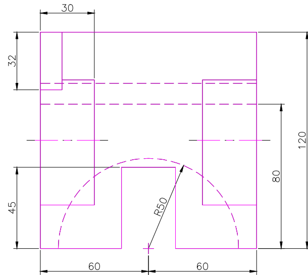
FRONT SCALE 1/2
