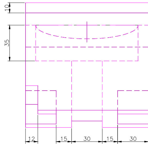
TOP SCALE 1/2
