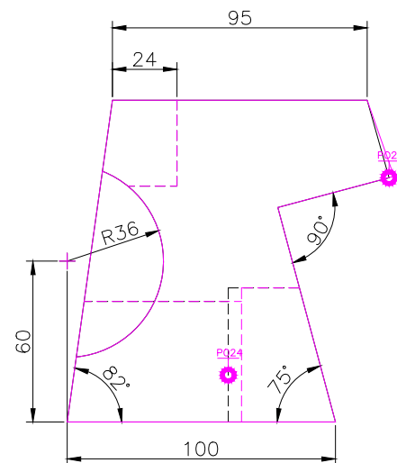
RIGHT SCALE 1/2
