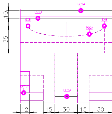
TOP SCALE 1/2
