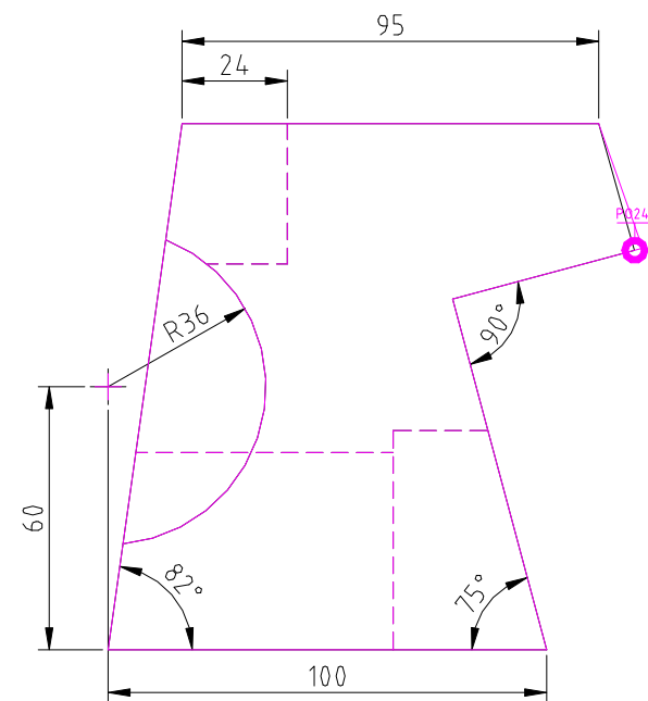
RIGHT SCALE 1/2
