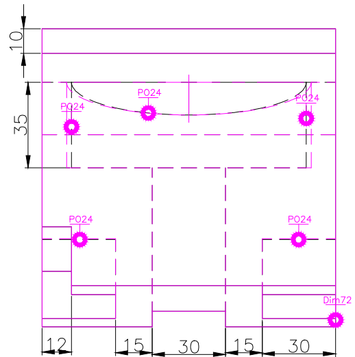
TOP SCALE 1/2
