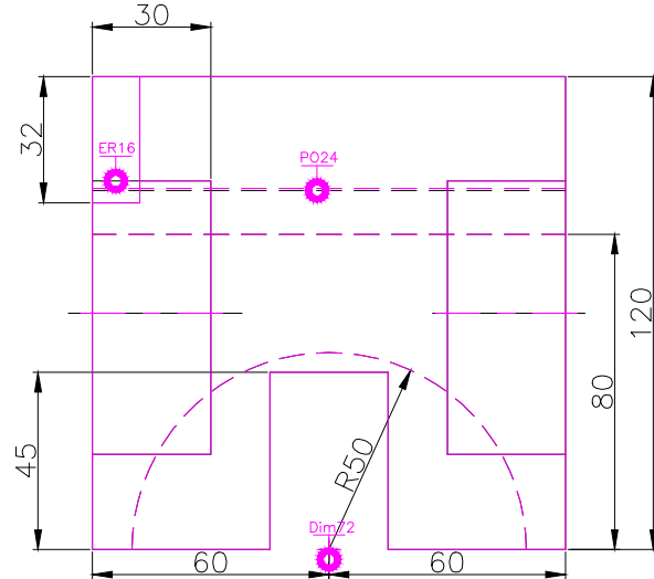
FRONT SCALE 1/2
