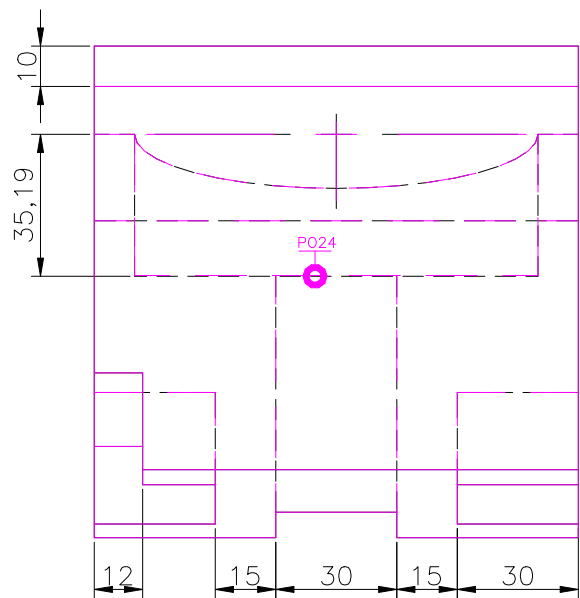
TOP SCALE 1/2
