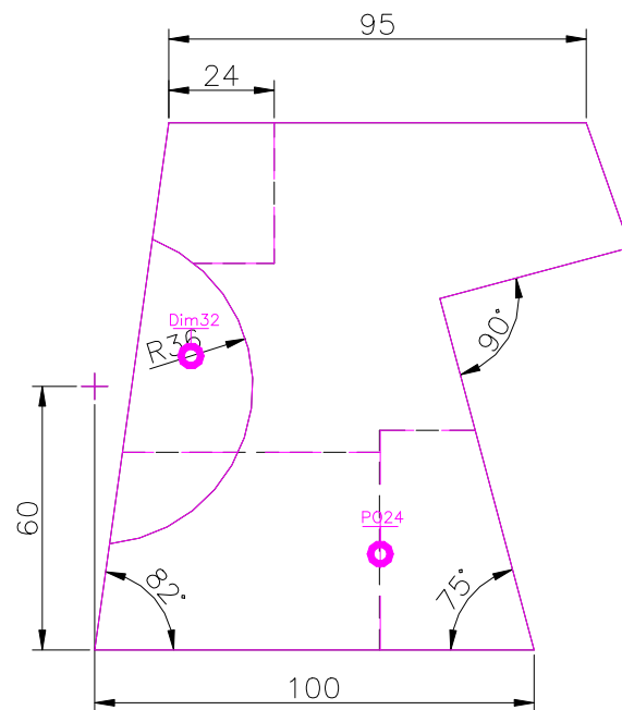
RIGHT SCALE 1/2
