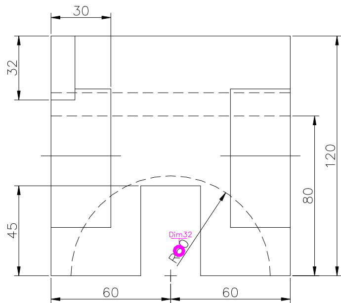
FRONT SCALE 1/2
