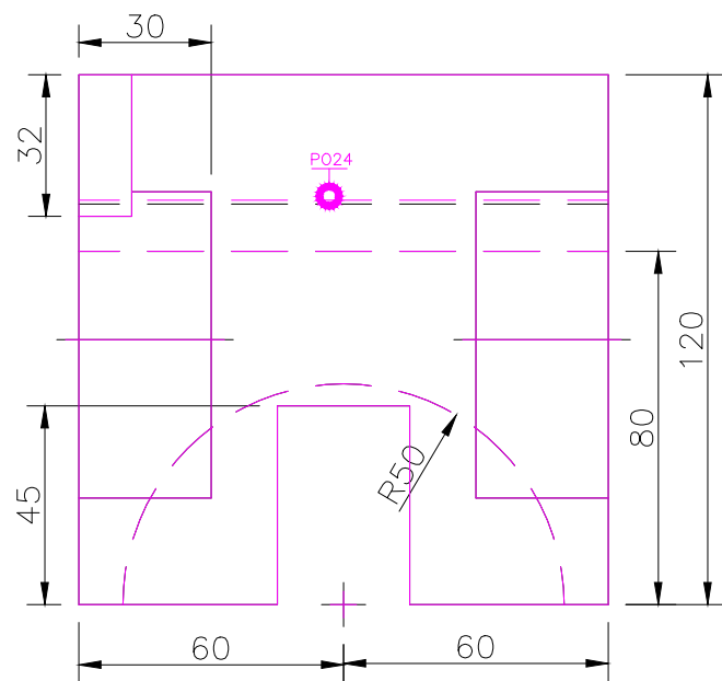
FRONT SCALE 1/2
