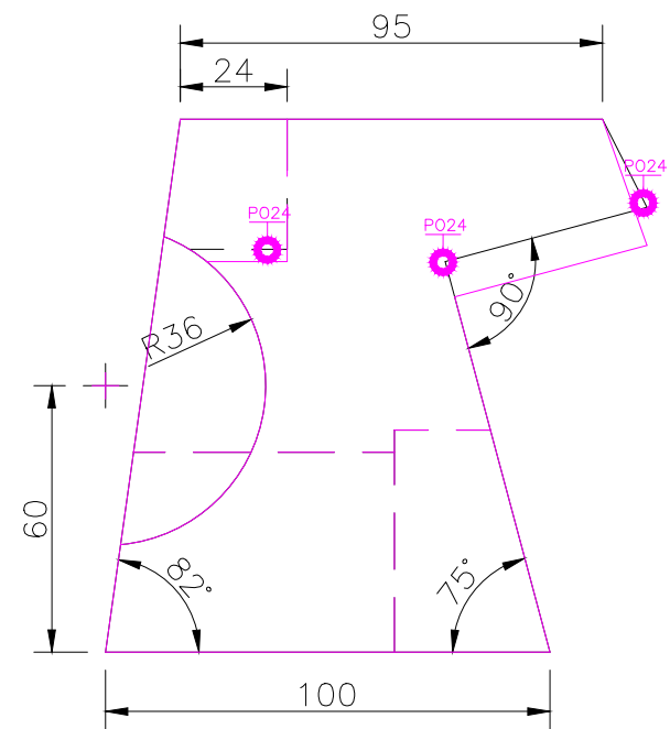
RIGHT SCALE 1/2
