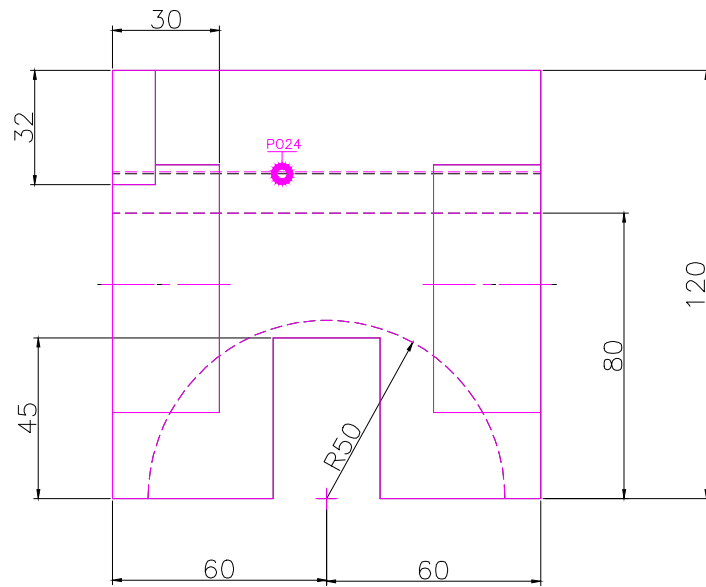
FRONT SCALE 1/2
