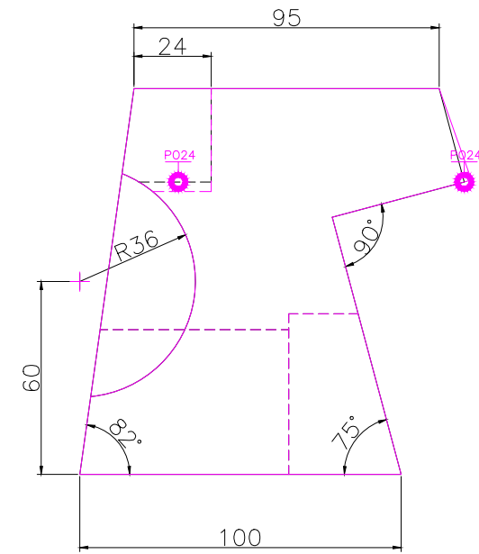
RIGHT SCALE 1/2
