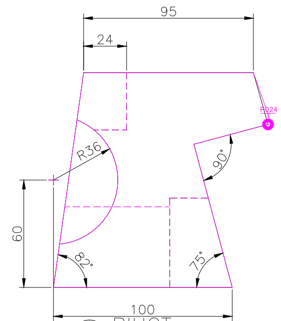
RIGHT SCALE 1/2
