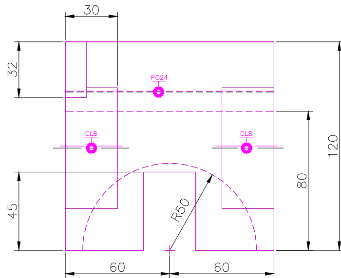
FRONT SCALE 1/2
