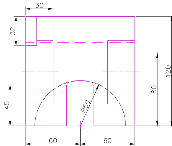
FRONT SCALE 1/2
