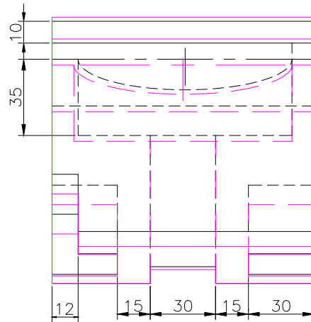
TOP SCALE 1/2
