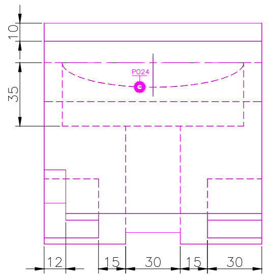
TOP SCALE 1/2
