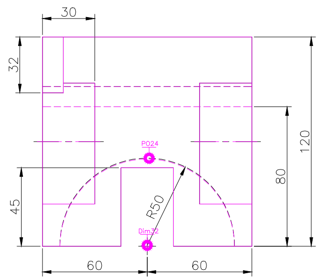
FRONT SCALE 1/2
