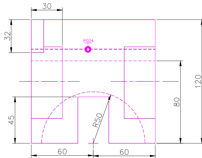
FRONT SCALE 1/2
