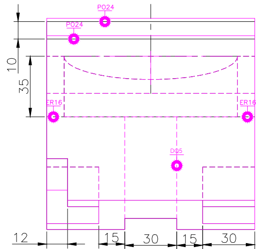
TOP SCALE 1/2
