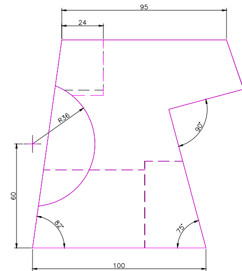
RIGHT SCALE 1/2
