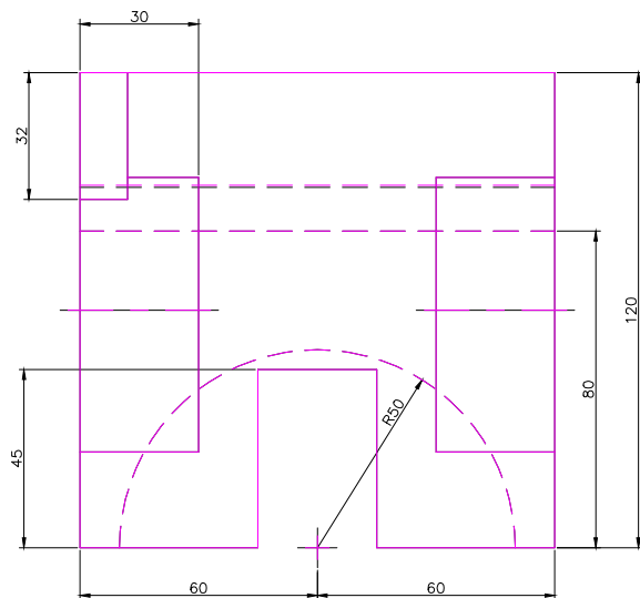
FRONT SCALE 1/2
