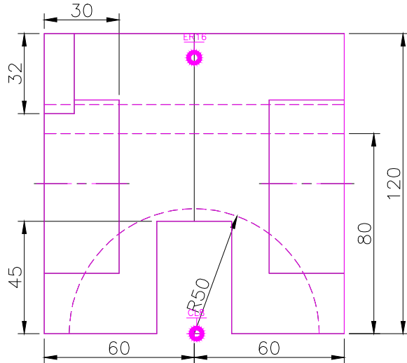
FRONT SCALE 1/2
