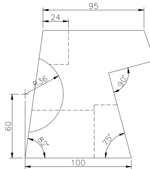
RIGHT SCALE 1/2
