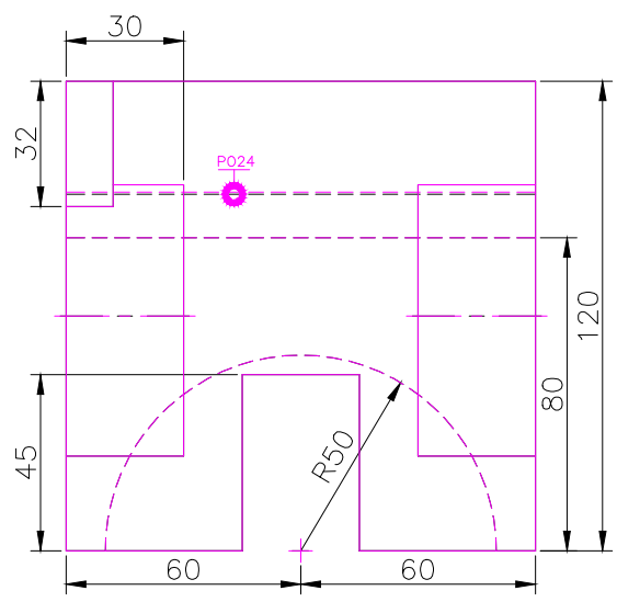
FRONT SCALE 1/2
