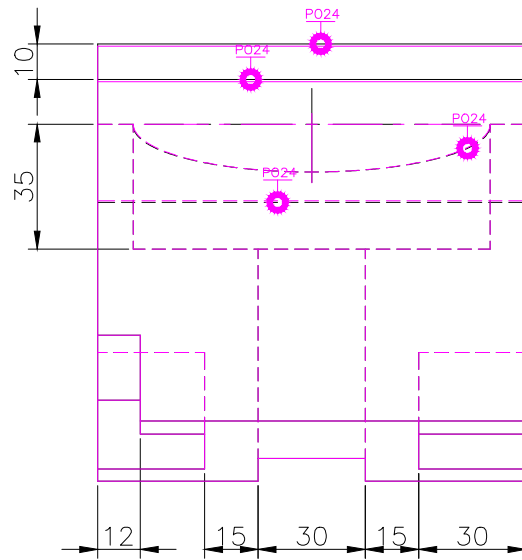
TOP SCALE 1/2
