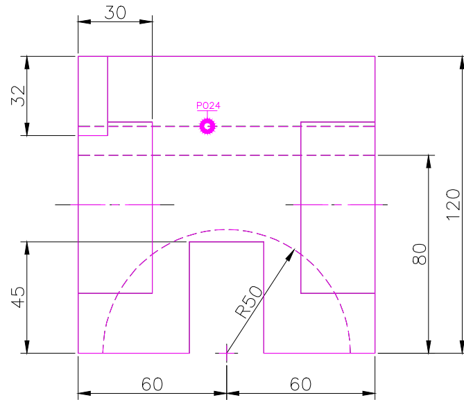
FRONT SCALE 1/2
