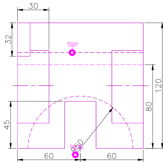
FRONT SCALE 1/2
