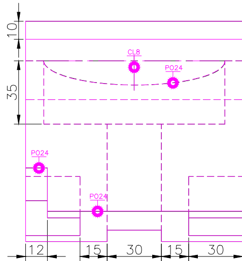
TOP SCALE 1/2
