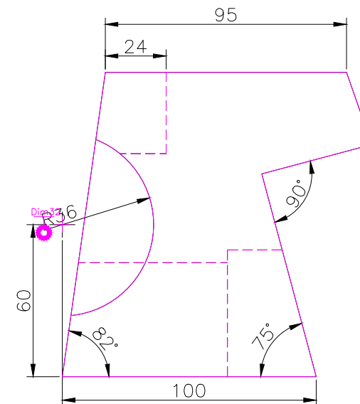
RIGHT SCALE 1/2
