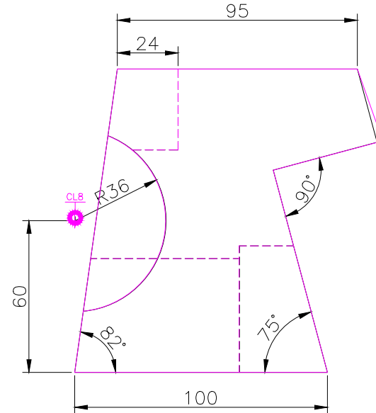
RIGHT SCALE 1/2
