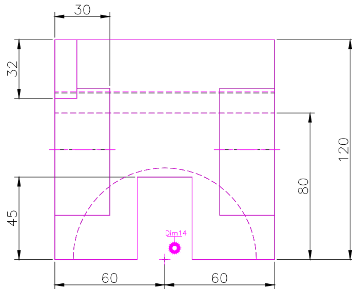
FORNT SCALE 1/2
