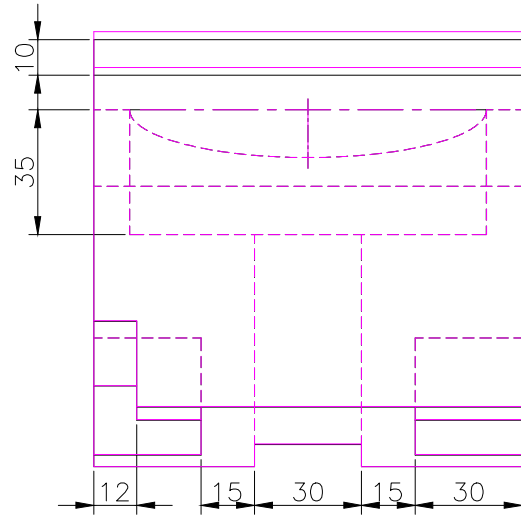
TOP SCALE 1/2
