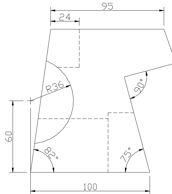
RIGHT SCALE 1/2
