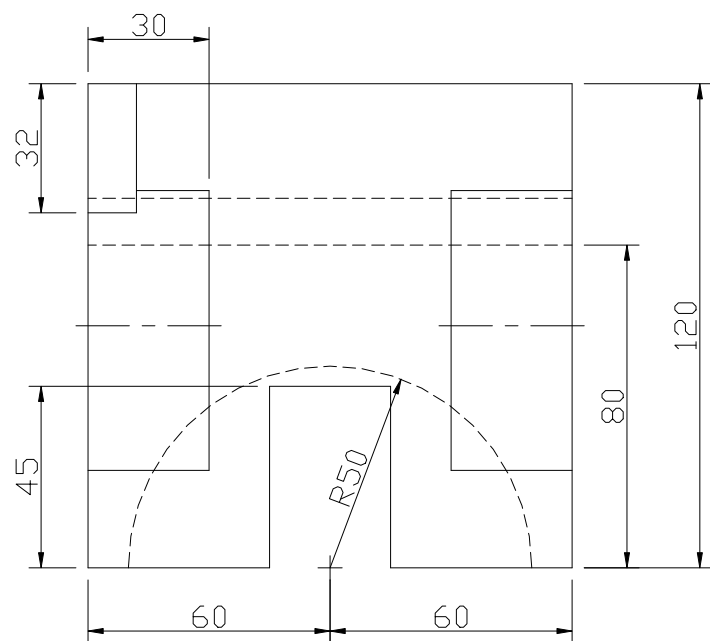
FRONT SCALE 1/2
