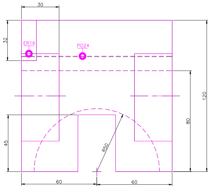
FRONT SCALE 1/2
