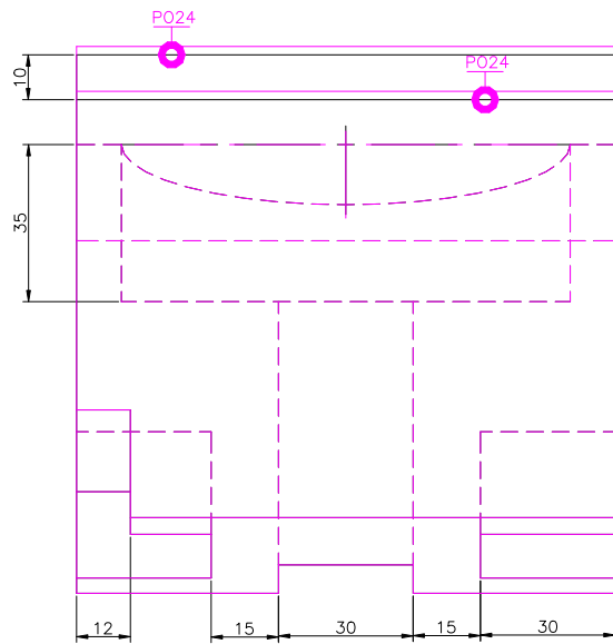
TOP SCALE 1/2
