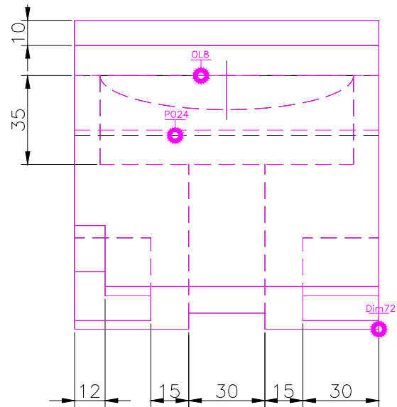
TOP SCALE 1/2
