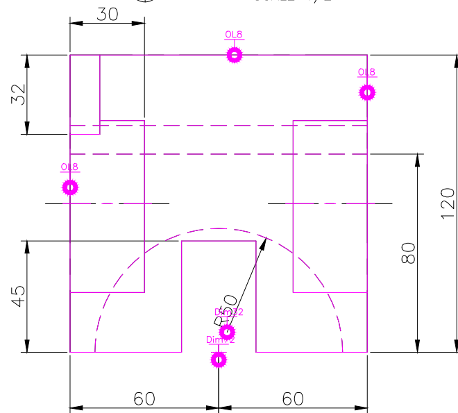
FRONT SCALE 1/2
