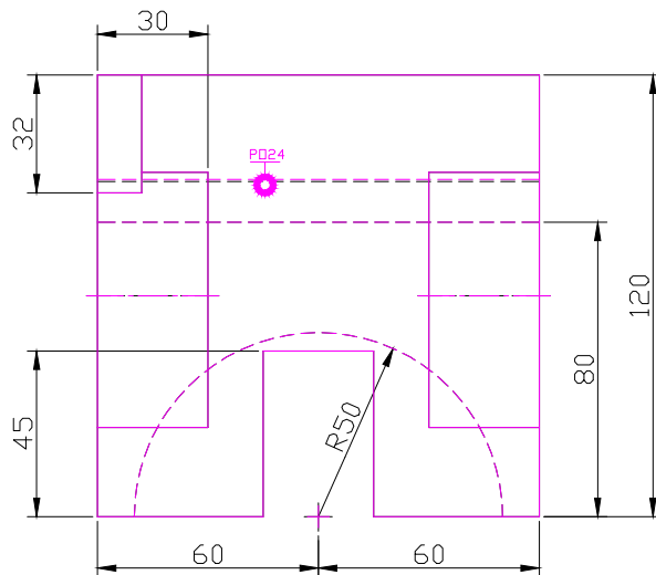
FRONT SCALE 1/2
