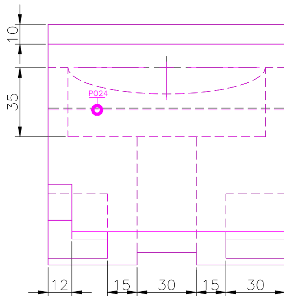
TOP SCALE 1/2
