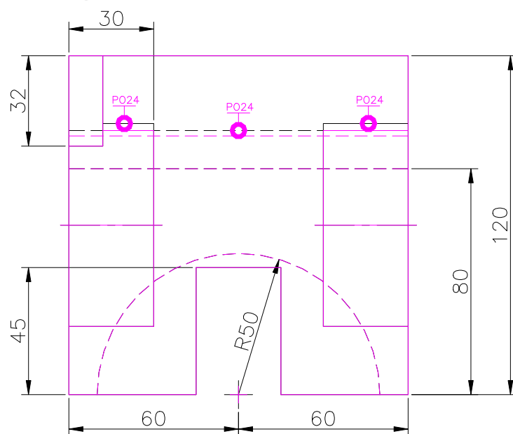
FRONT SCALE 1/2
