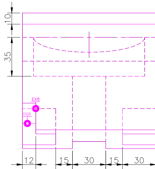
TOP SCALE 1/2
