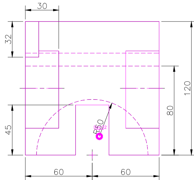
FRONT SCALE 1/2
