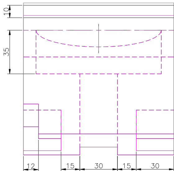
TOP SCALE 1/2
