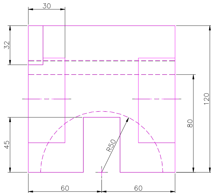
FRONT SCALE 1/2
