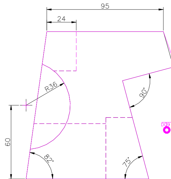
RIGHT SCALE 1/2
