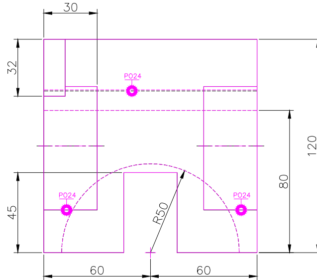
FRONT SCALE 1/2
