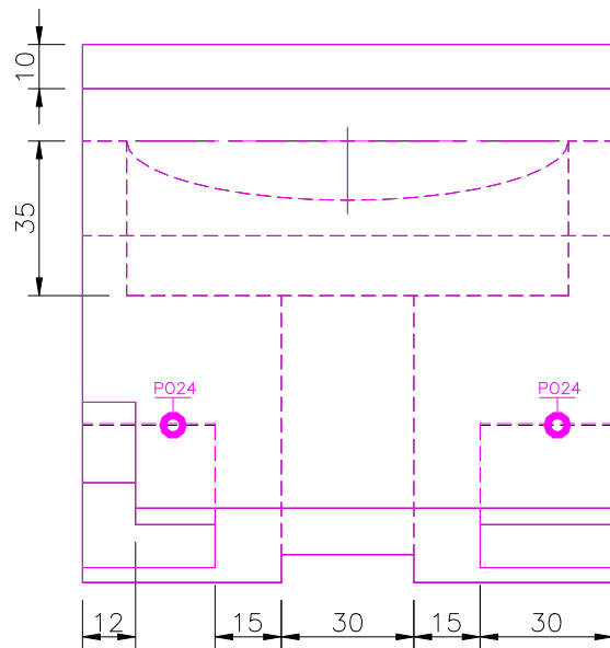
TOP SCALE 1/2
