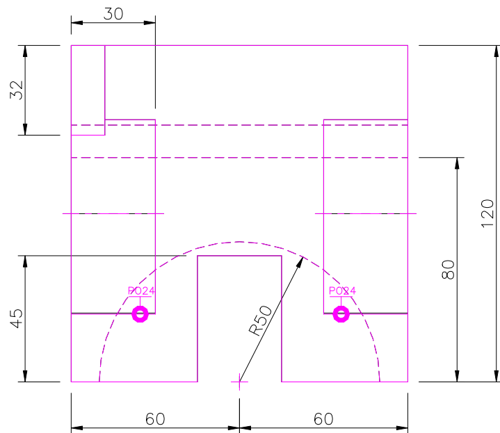
FRONT SCALE 1/2
