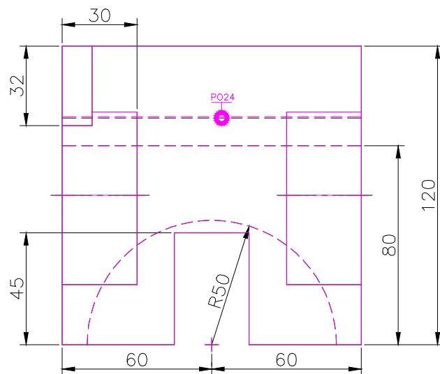
FRONT SCALE 1/2
